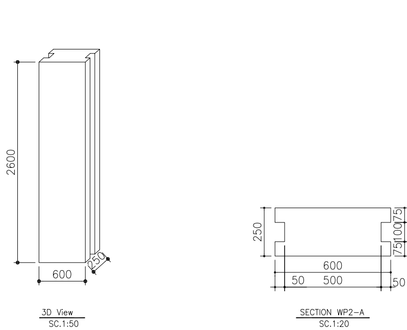
AAC. Wall panel WP-02 600x2600 mm N=120
