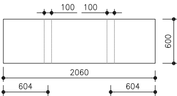
TYPE ST-04 SC.1:50
