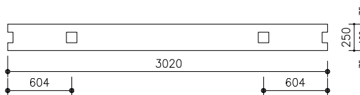
TYPE ST-01 SC.1:50
