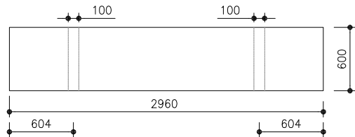
TYPE ST-05 SC.1:50
