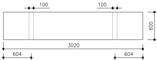
TYPE ST-01 SC.1:50
