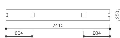
TYPE ST-06 SC.1:50
