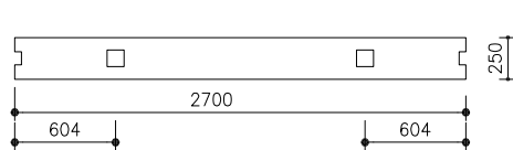
TYPE ST-02 SC.1:50
