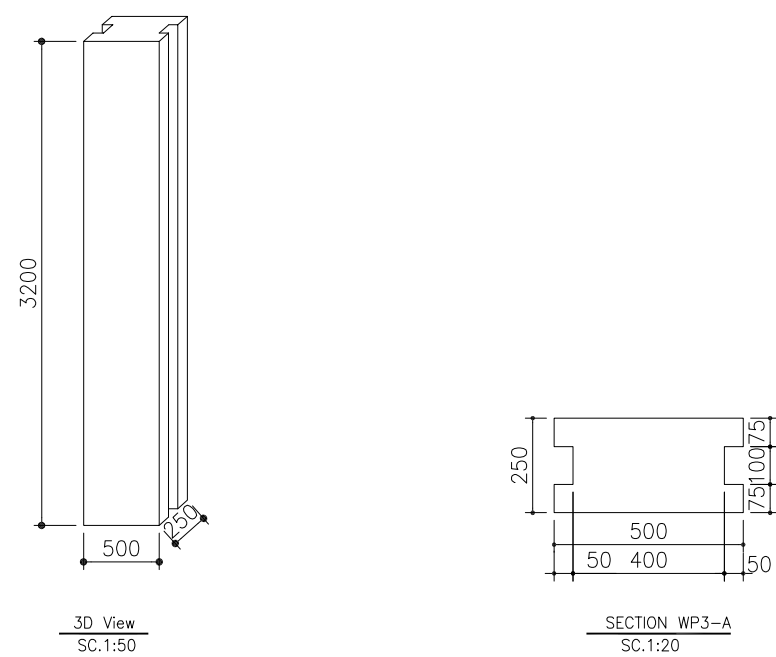
AAC. Wall panel WP-03 500x3200 mm N=60
