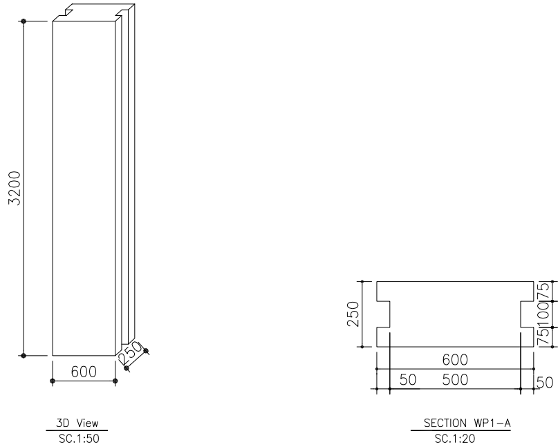
AAC. Wall panel WP-01 600x3200 mm N=487
