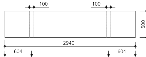
TYPE ST-03 SC.1:50
