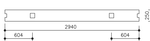
TYPE ST-03 SC.1:50
