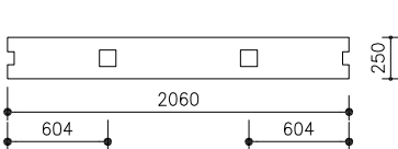
TYPE ST-04 SC.1:50
